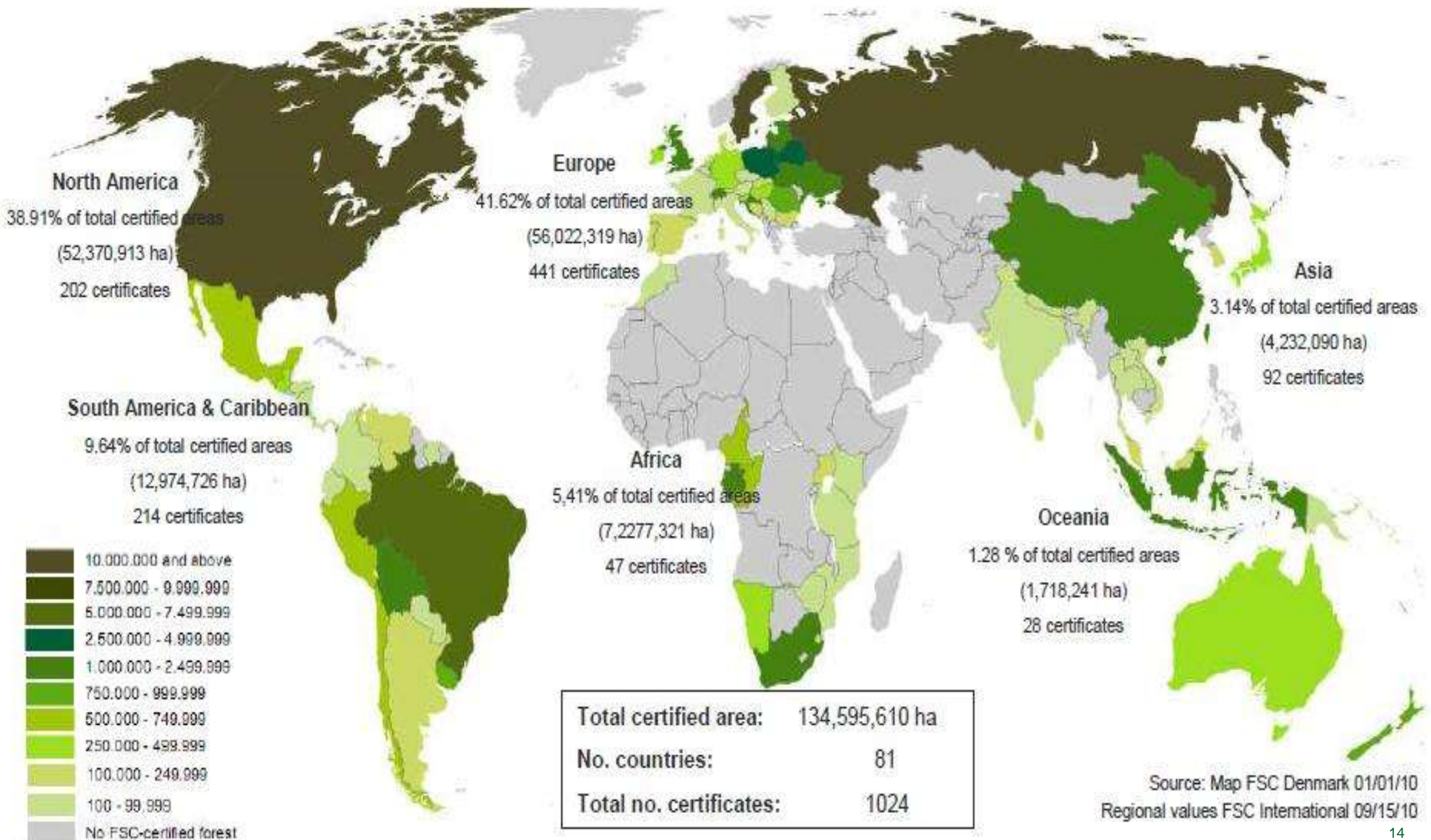
Global FSC certified forest area: by region
